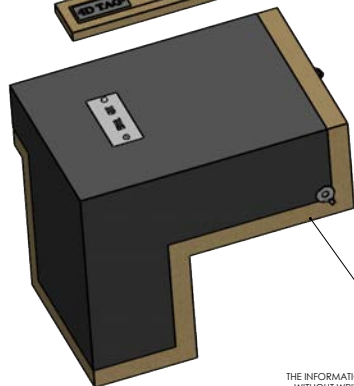
Manifold Cover Part #: 3242710
